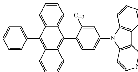
[Chemical Formula 9]
