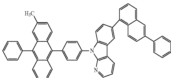
(Compound 2)
