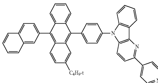
(Compound 7)
