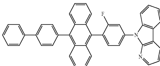
(Compound 8)
