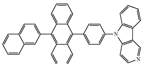
[Chemical Formula 6]
