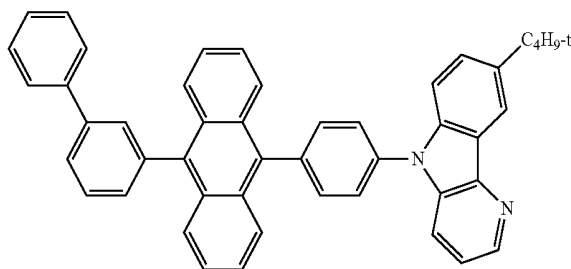
(Compound 4)
