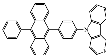
[Chemical Formula 3]
