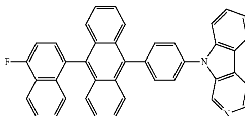
[Chemical Formula 5]
